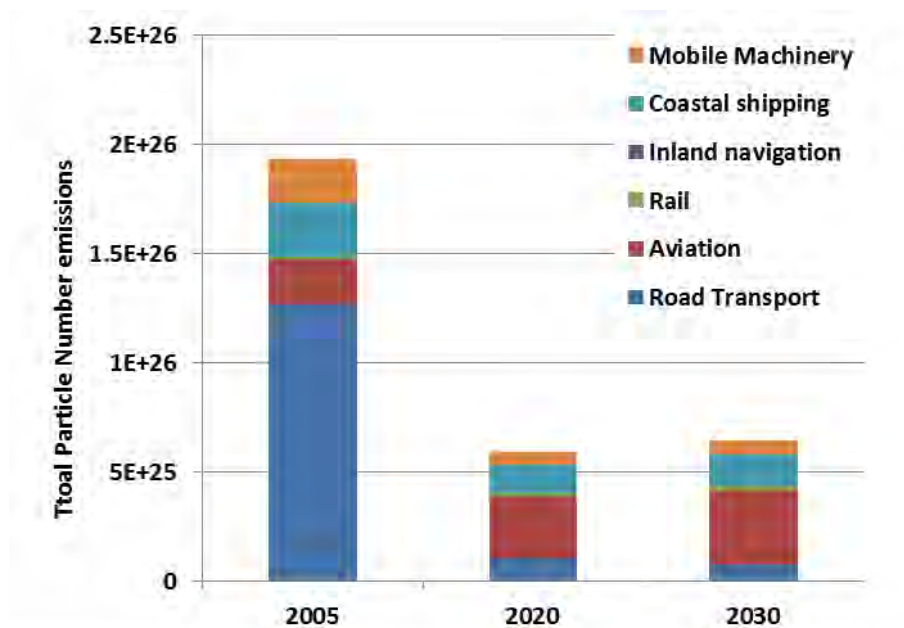
Figure 10. U.K. transport sector total particle number emissions in 2005, 2020 and 2030 excluding International shipping. (Aviation = airport LTO's up to 1000 m) (data from TNO).
