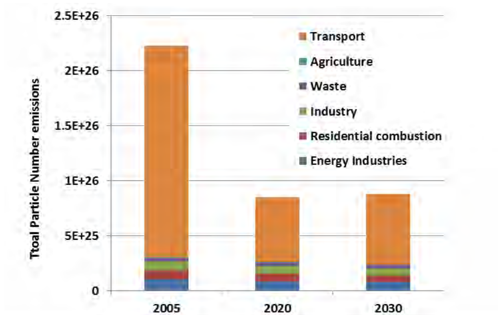
Figure 9. Total particle number emissions for 2005, 2020 and 2030 for the UK by source sector (data from TNO).
